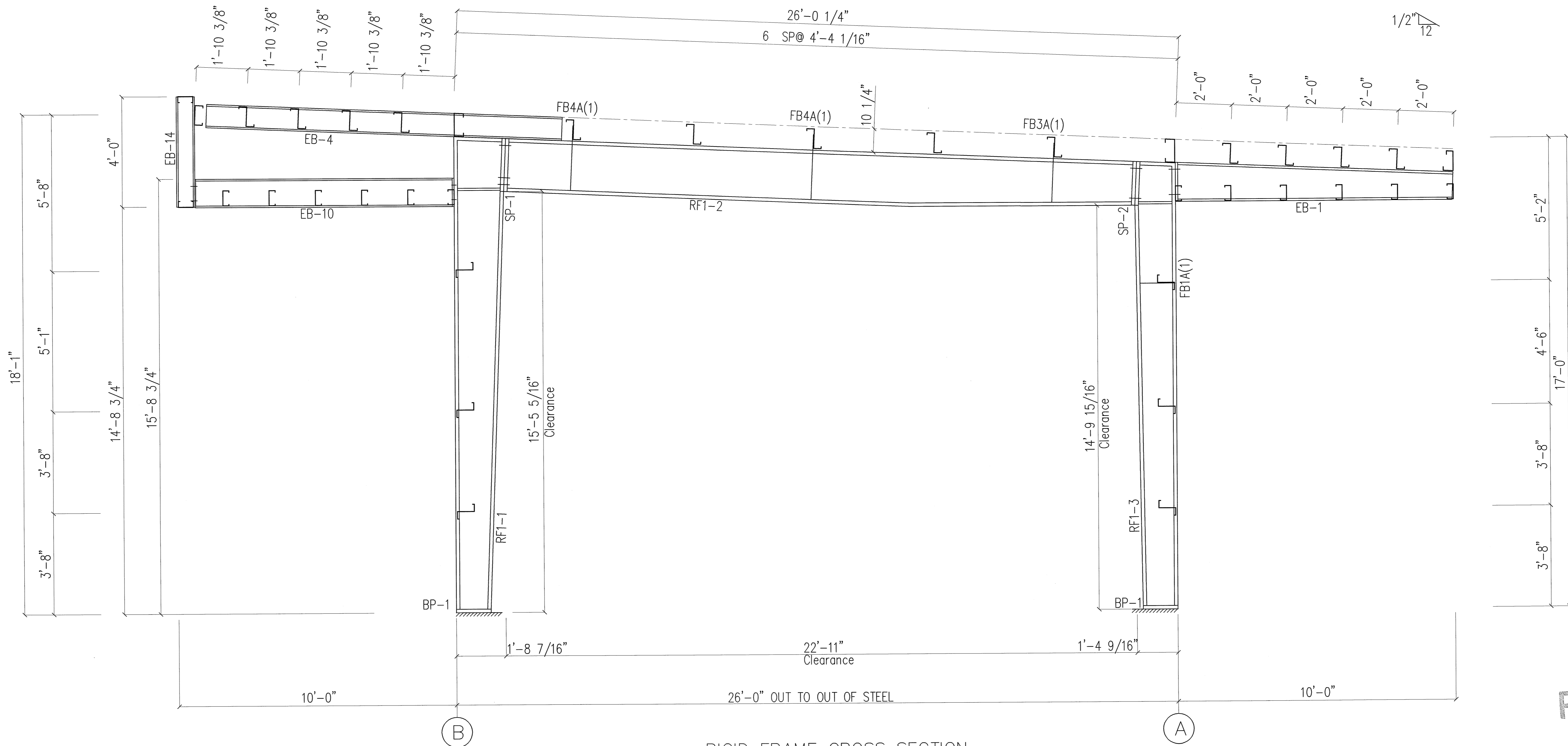
RIGID FRAME CROSS SECTION FOR FRAME LINE 1 3
