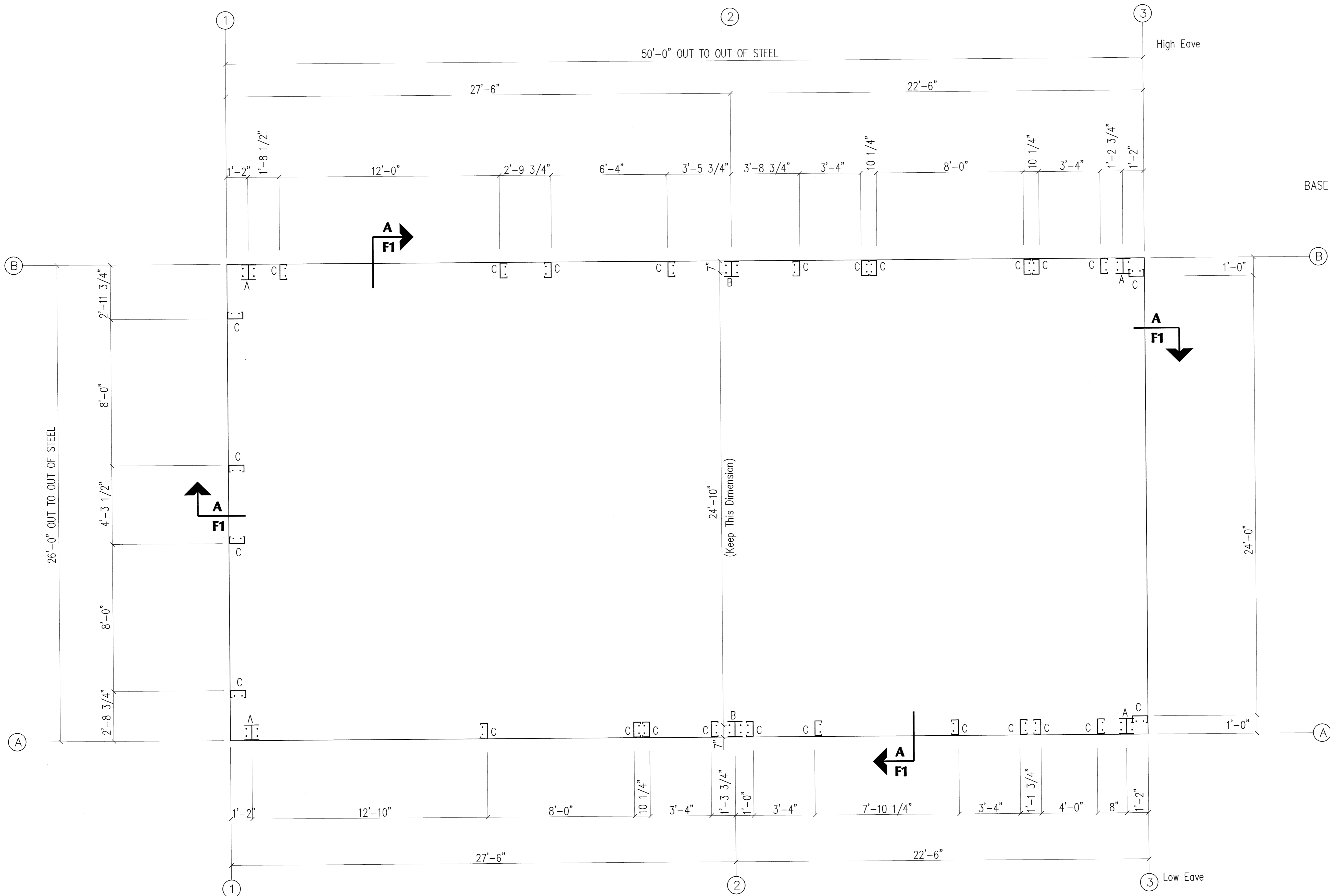
COLUMN LAYOUT PLAN NOTE: All Base Plates @ 100'-0" (U.N.)
