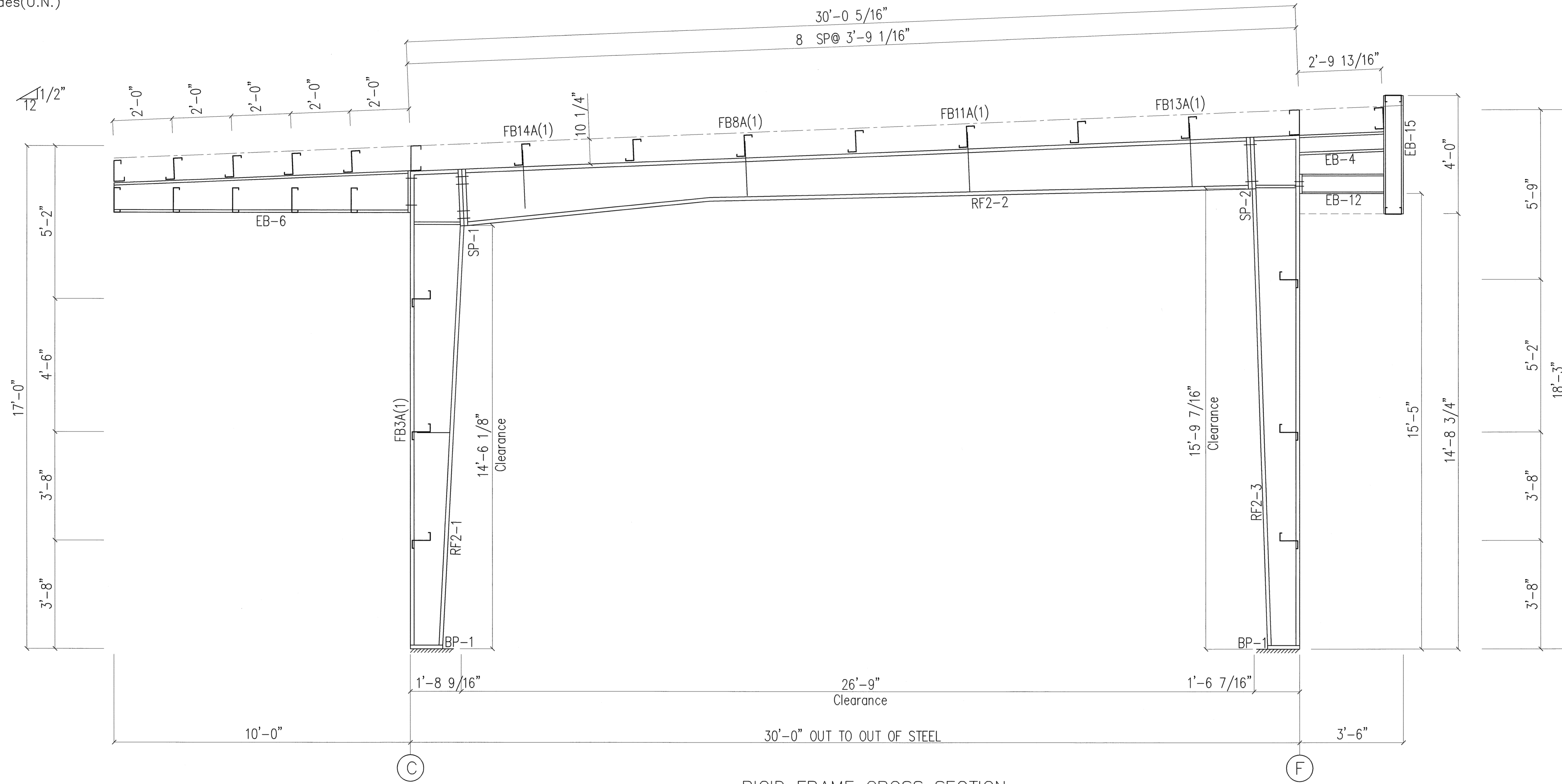
RIGID FRAME CROSS SECTION FOR FRAME LINE 3 4 5
