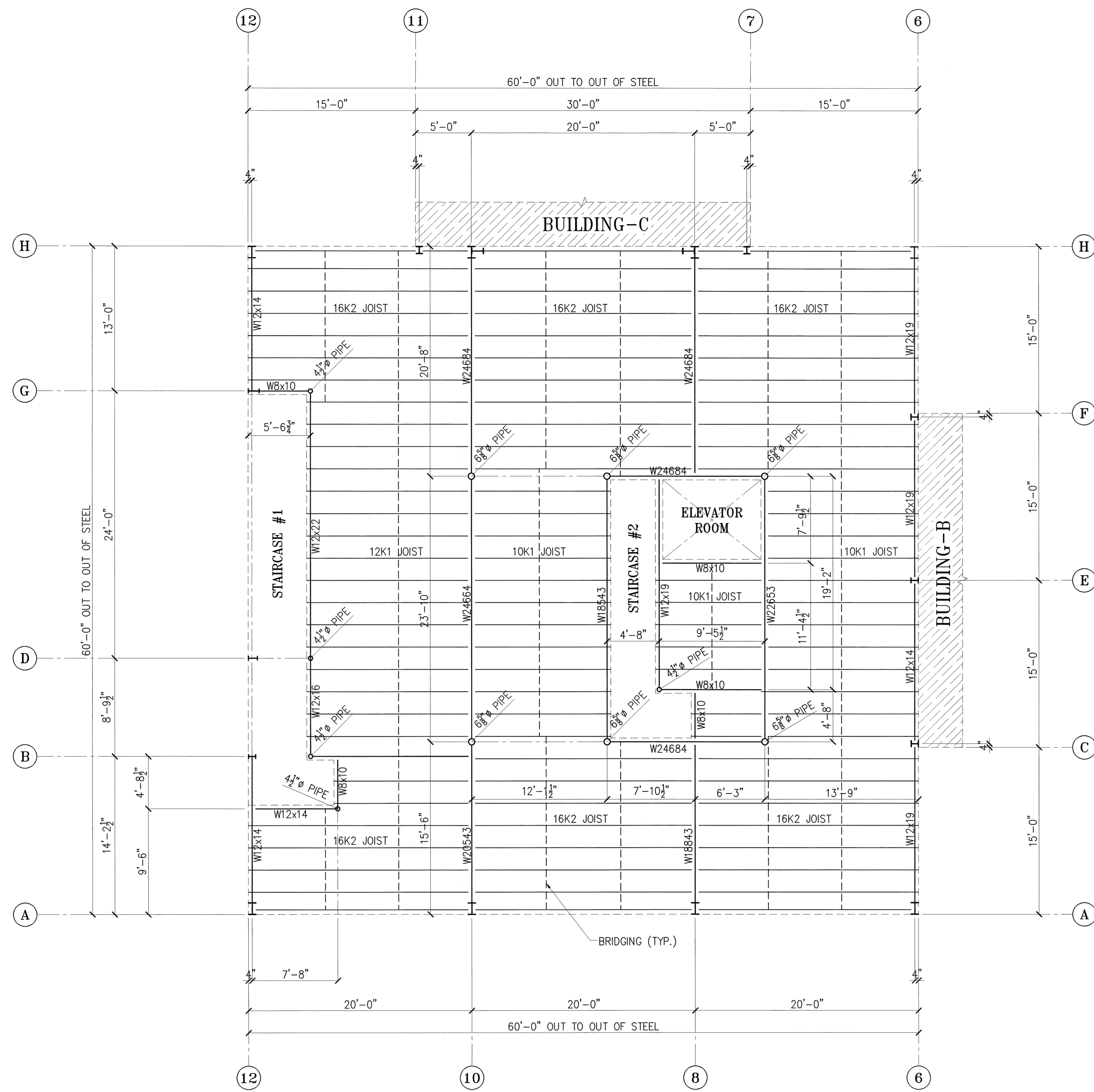
MEZZANINE FLOOR FRAMING PLAN
